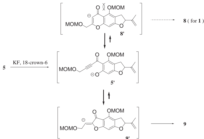
Scheme 6. Cyclization mechanism of 1-(dihydrobenzofuran-5-yl)butynone 5 .
