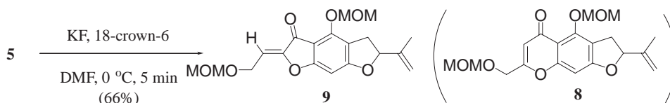
Scheme 5. Cyclization of 1-(dihydrobenzofuran-5-yl)butynone 5 in Nakatani's procedure.
