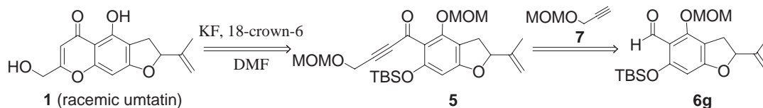
Scheme 3. Synthetic strategy for racemic umtatin 1.
