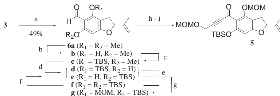
Scheme 3. Synthetic strategy for racemic umtatin 1.
