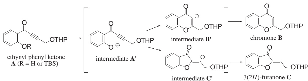
Scheme 2. Construction of 2-(hydroxymethyl)chromones.
