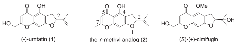
Figure 1. Chiral (–)-umtatin ( 1 ), the 7-methyl analog 2 , and chiral (+)-cimifugin.
