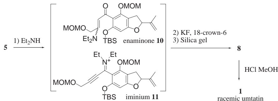
Scheme 8. Revised cyclization of 1-(dihydrobenzofuran-5-yl)butynone 5 .
